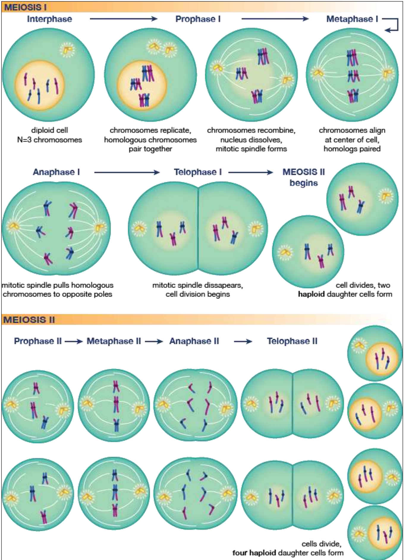
Diagrammatic representation of different stages of meiosis
