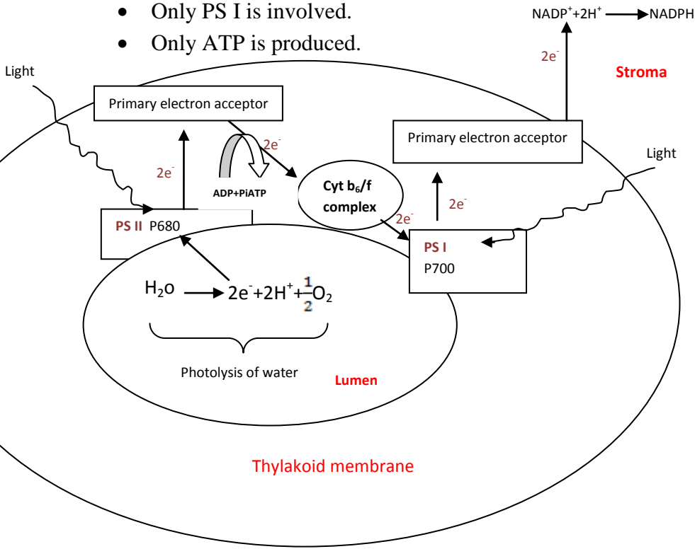
Z-Scheme of electron transport/ non cyclic
