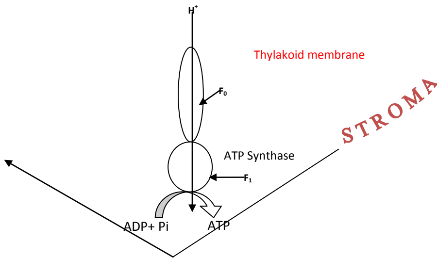
Schematic representation of chemiosmotic hypothesis
